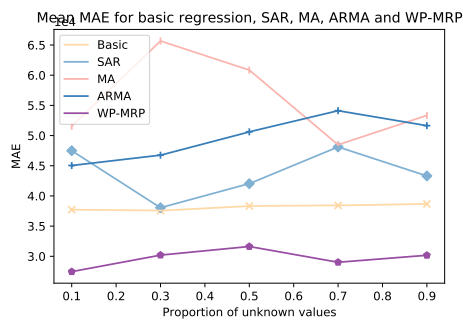
Figure 8.23: Mean MAE as a function of p for GDP interpolation trained on Seoul and tested on Daegu: (spatial) regression methods.
