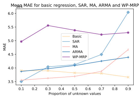
Figure 8.3: Mean MAE as a function of p for GDP interpolation trained on Taipei and tested on Taipei: (spatial) regression methods.
