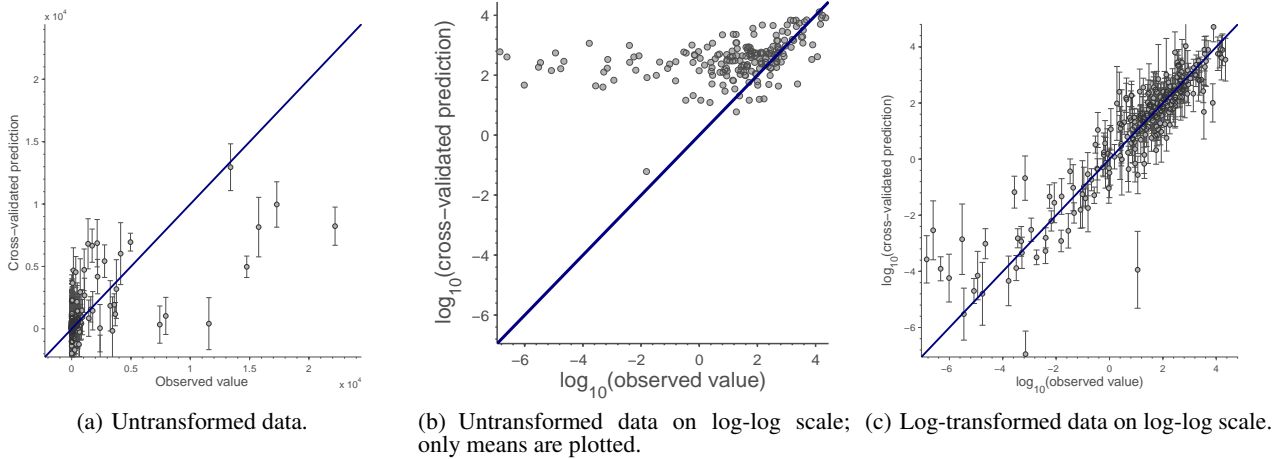
Figure 2: Performance of noise-free Gaussian process models for CMA-ES-sphere based on an initial design using a random LHD; in (a) and (c) we plot mean \pm one standard deviation of the prediction. Metrics: (a) RMSE=2.289, CC=0.329, LL=-8.274, 22 points predicted below zero; (c) RMSE=0.858, CC=0.927, LL=-1.407. For better visual comparison to (c), (b) shows exactly the same mean predictions as (a), but on a loglog scale, for the data points predicted above zero.
