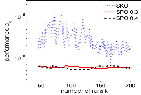
Figure 1: Comparison of SKO and two variants of SPO (discussed in Section 5.1) for optimising CMA-ES on the Sphere function. We plot the performance p_k of each method (mean solution quality CMA-ES achieved in 100 test runs on the Sphere function using the method’s chosen parameter settings) as a function of the number of algorithm runs, k , it was allowed to perform; these values are averaged across 25 runs of each method.
