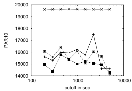
(f) Application - Reduced Training Cutoff Time
