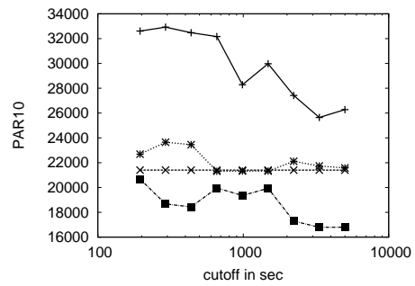
(d) Crafted - Reduced Training Cutoff Time
