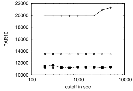
(b) Random - Reduced Training Cutoff Time
