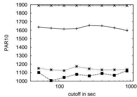
(h) ASP-Set - Reduced Training Cutoff Time
