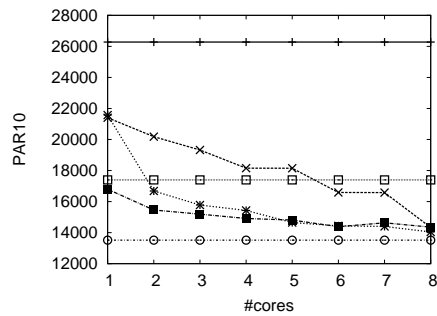
(c) Crafted - Parallel Schedule
