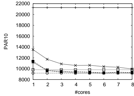
(a) Random - Parallel Schedule
