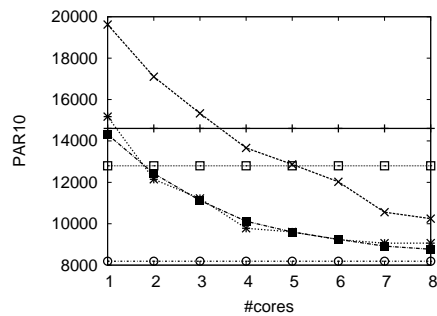
(e) Application - Parallel Schedule
